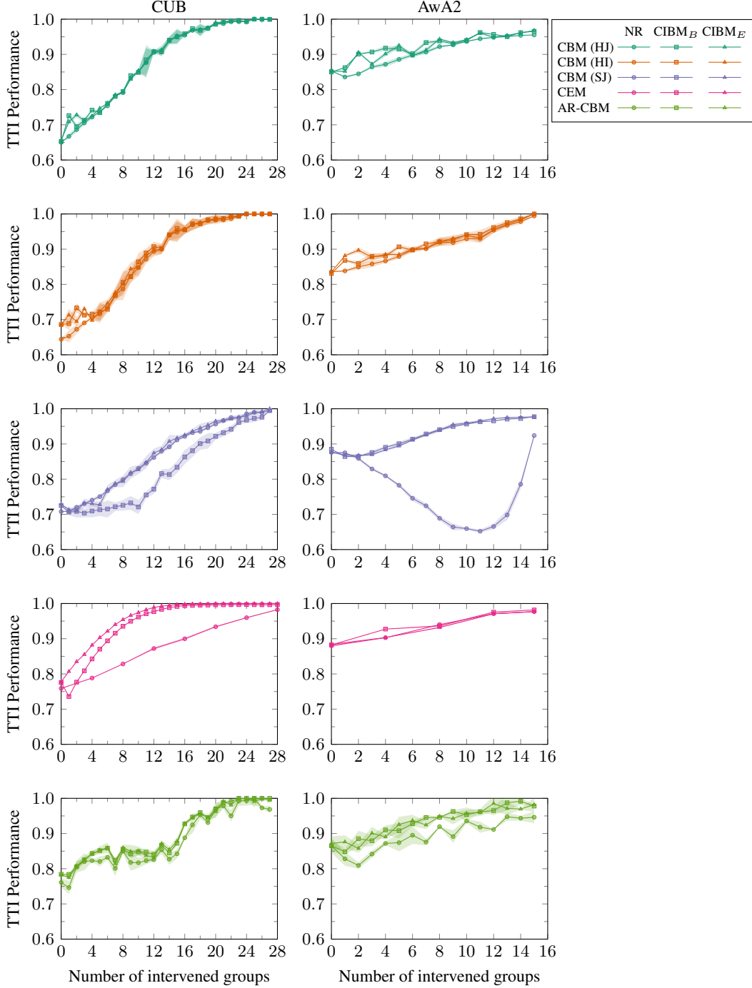
Figure C.1: Expanded results from Fig. 3. Change in target prediction accuracy after intervening on concept groups following the random strategy as described in Section 4.3. (TTI stands for Test-Time Interventions and NR for non-regularized.)
