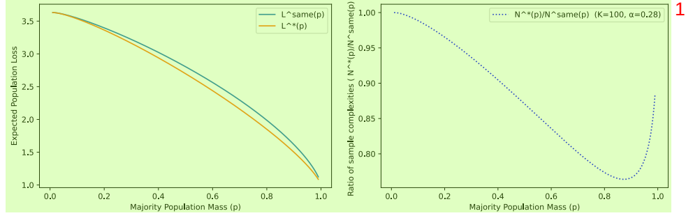
Figure 2: We consider the setup of Corollary 3.3 with A = 1 , \alpha = 0.28 , K = 100 , and some fixed N . On the left plot, we show the "non-shifted" expected population loss L^{\text{same}}(p) and the optimally mixed expected population loss L^*(p) as a function of majority population mass p . On the right plot, we show the ratio of sample complexities for any fixed \epsilon > 0 , N_{\epsilon}^{\text{ratio}}(p) as a function of the mass of the majority population, p . We can see significant improvement in the sample complexity from the positive distribution shift from using optimal mixing ratio, even up to \approx 25\% .
