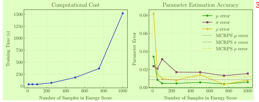
Figure A2: Computational cost versus parameter estimation accuracy for the energy score with varying sample sizes. The left panel shows training time across different numbers of Monte Carlo samples, while the right panel displays absolute errors in parameter estimates ( \mu , \sigma , \rho ), with dashed lines indicating the corresponding MVG-CRPS reference values.
