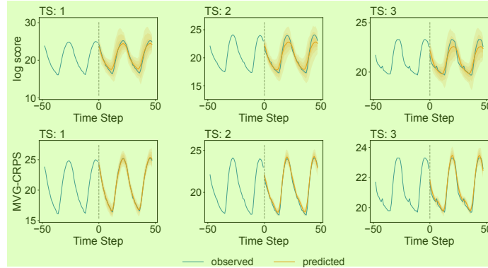
Figure A4: Comparison of probabilistic forecasts from N-HiTS on the m4_hourly dataset. 6
