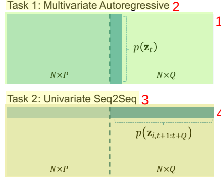
Figure 2: Illustration of the multivariate autoregressive and univariate Seq2Seq forecasting tasks. 5
