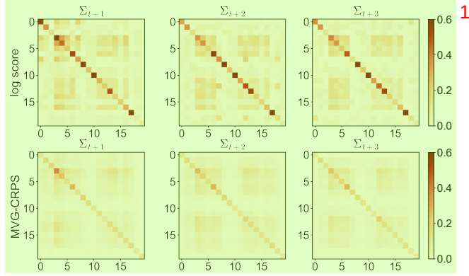
Figure 4: Comparison of output covariance matrices \Sigma_t from GPVar on the elec_weekly dataset. For visual clarity, covariance values are clipped between 0 and 0.6.
