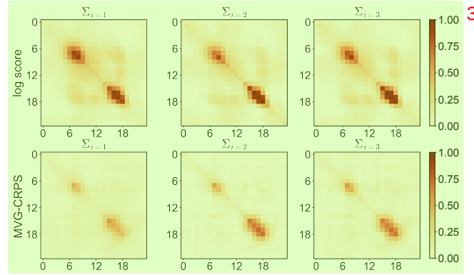
Figure A3: Comparison of output covariance matrices \Sigma_i from N-HiTS on the traffic dataset. For 4 visual clarity, covariance values are clipped between 0 and 1.0.
