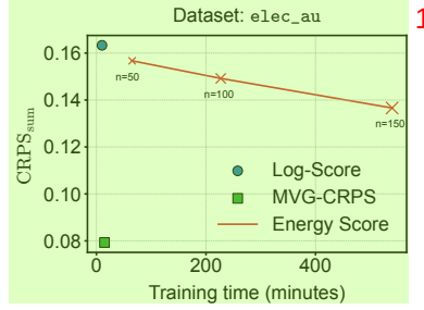
Figure 1: An example showing MVG-CRPS achieves better accuracy and faster training by avoiding sampling and reducing sensitivity to outliers. ES results are shown for different sample sizes.
