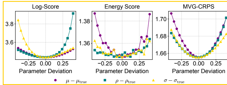
Figure 3: Sensitivity of scoring rules to parameter deviations in the predicted mean, standard deviation, and correlation coefficient from the true data distribution \mu_{\text{true}} = 1, \sigma_{\text{true}} = 1, \rho_{\text{true}} = 0.4 . The ES values are computed with a sample size of 500.
