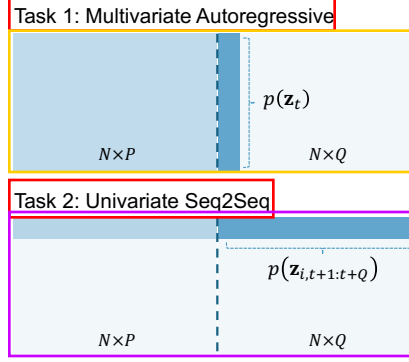
Figure 2: Illustration of the multivariate autoregressive and univariate Seq2Seq forecasting tasks.
