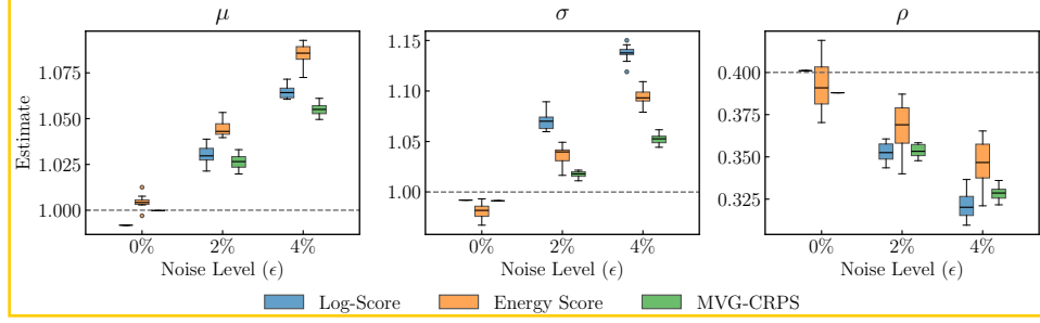
Figure A1: Parameter recovery under data contamination. Boxplots show the estimated parameters (\mu, \sigma, \rho) of a bivariate Gaussian distribution using three proper scoring rules across varying contamination levels. Dashed lines indicate the ground truth values. Each boxplot summarizes estimates from 10 independent runs with different random seeds for contamination.
