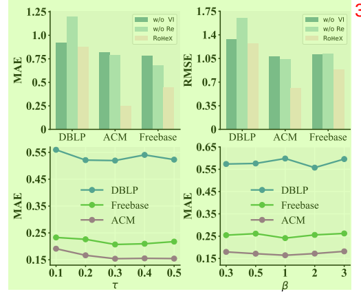
Figure 3: Ablation study on three datasets and the influence of hyperparameters \tau and \beta on RoHeX.
