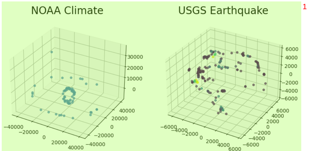
Figure 5: Visualizations for USGS Earthquake catalogue and NOAA Climate dataset. 2
