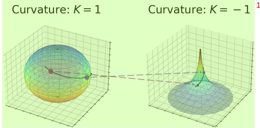
Figure 1: Mapping from spherical data into hyperbolic space.
