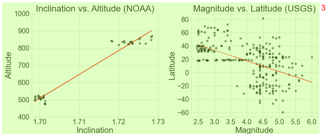
Figure 6: Heteroscedasticity in the NOAA and USGS datasets. 4
