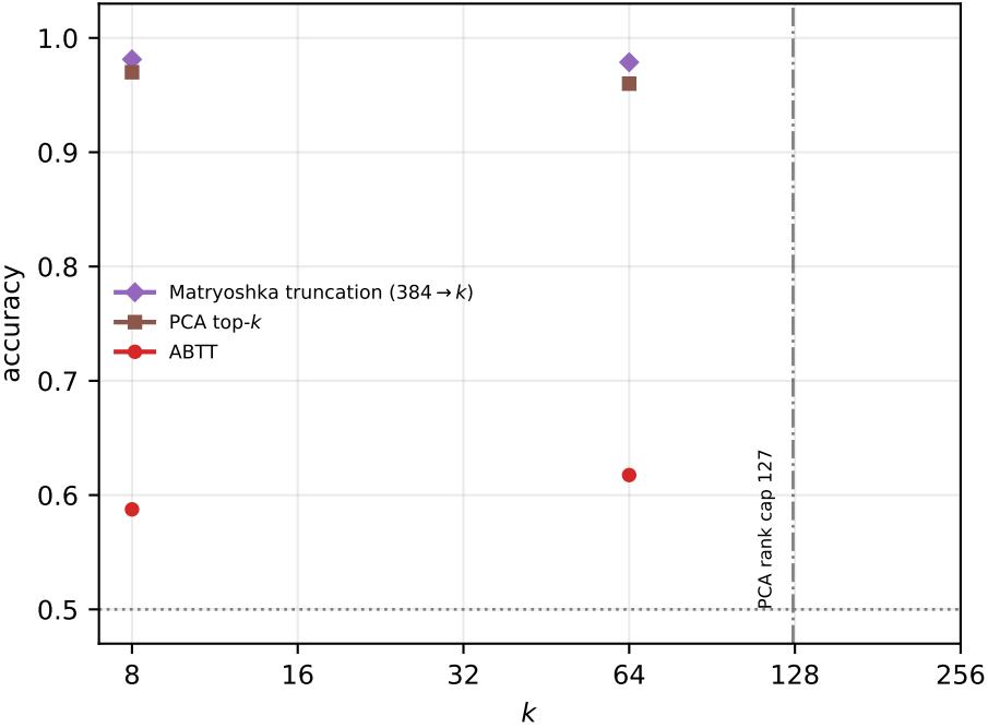
(f) bekko-a25m — Matryoshka vs PCA (PCA path capped at n_{tr} - 1 = 127 dims)
