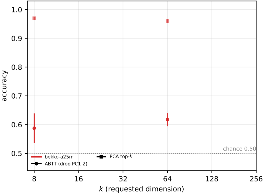
(d) Cross-lingual transfer — the regime where F10 reports ABTT to be decisive
