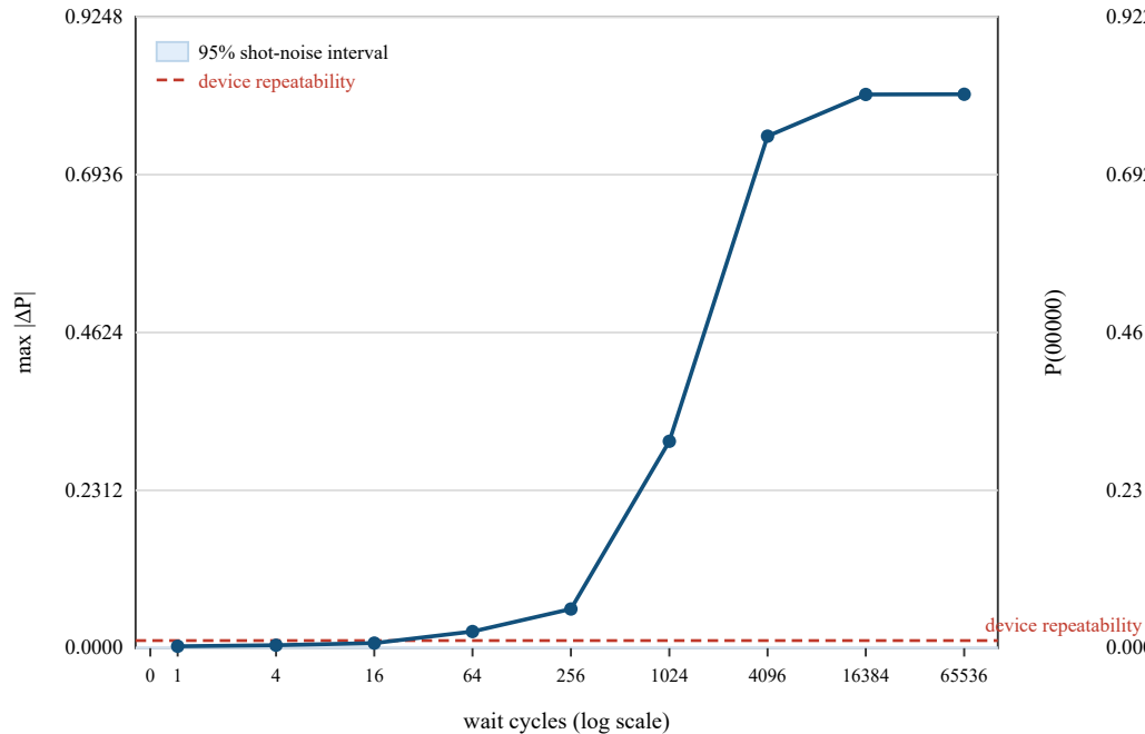
(a) deviation from the undelayed circuit
