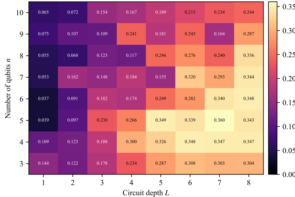
(b) Calibration error (ECE)
