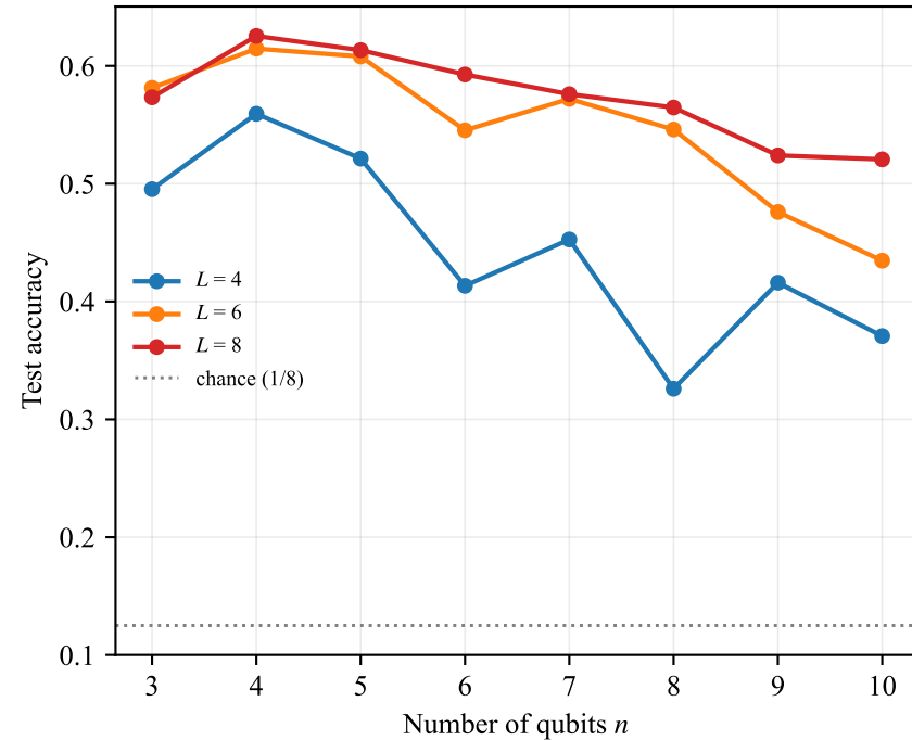
(c) Accuracy vs. n at fixed depth
