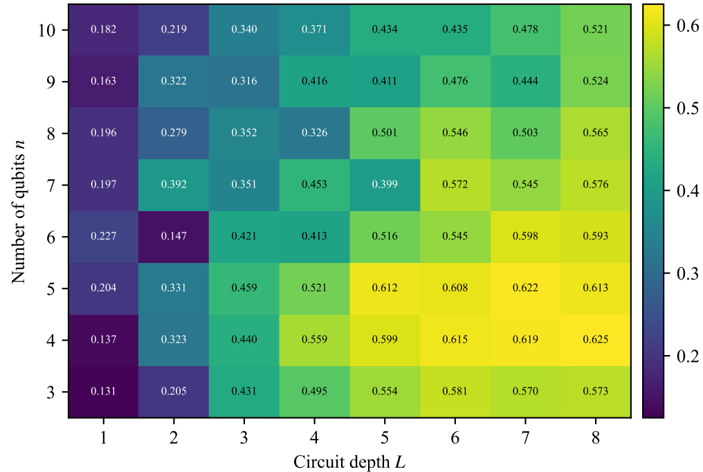
(a) Test accuracy over the (n, L) grid
