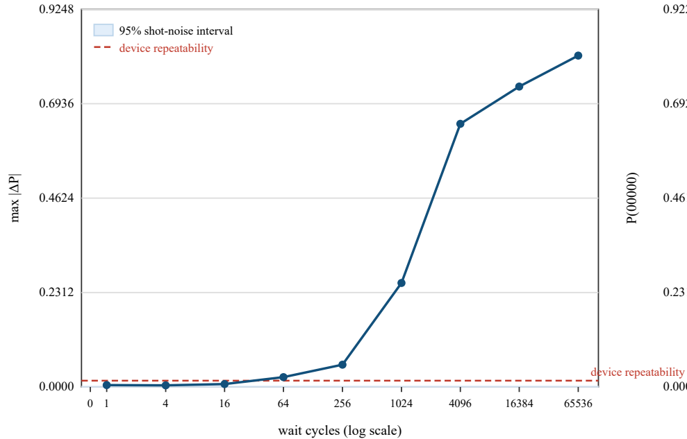
(a) deviation from the undelayed circuit
