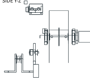
SIDE Y-Z
