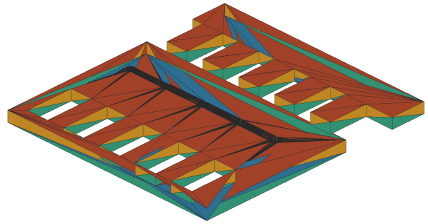
Figure 20: Cable topology overlay와 height-band slicing orientation preview
