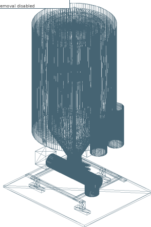
Figure 18: Dryer와 extruder hidden-line x-ray review
