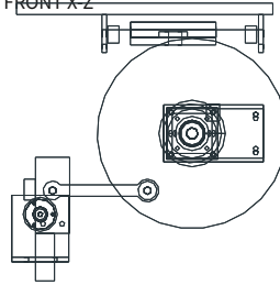
FRONT X-Z
