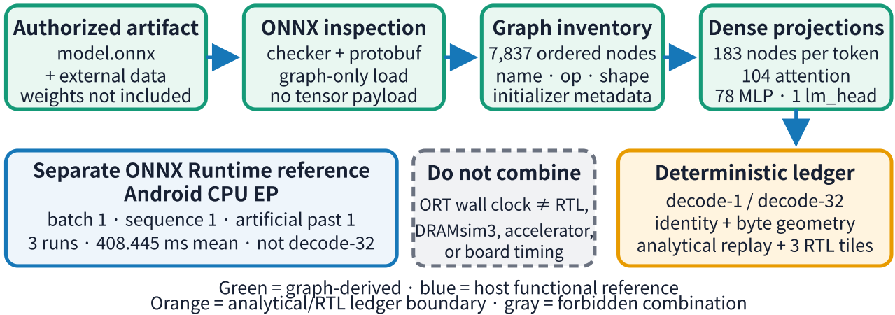
Figure 2 · ONNX graph and Runtime evidence boundary
