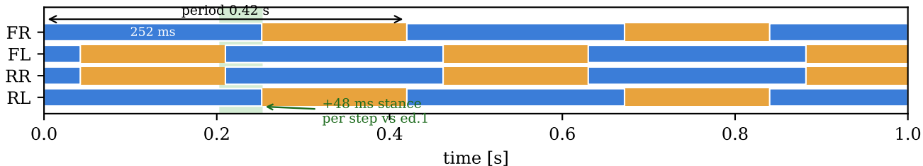
(b) edition 2 — platform retune (period 0.42 s, stance 252 ms)
