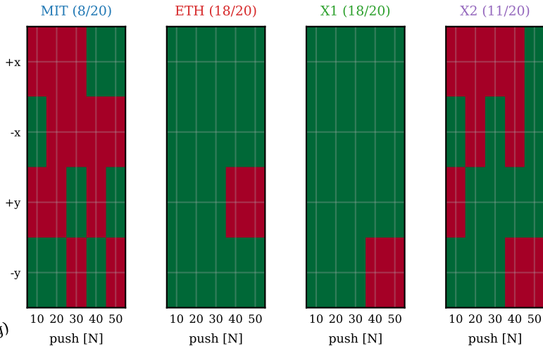
(b) S5 push recovery (green = recovered, 0.1 s impulse)
