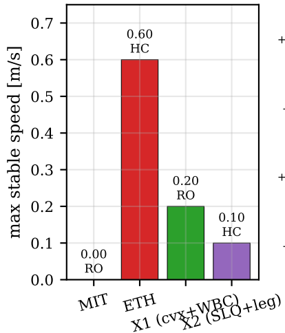
(a) S2 ramp-to-failure
