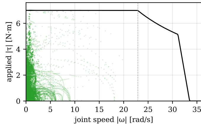
X1 (peak 189 rpm)
