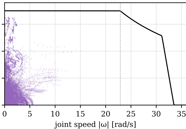
X2 (peak 144 rpm)
