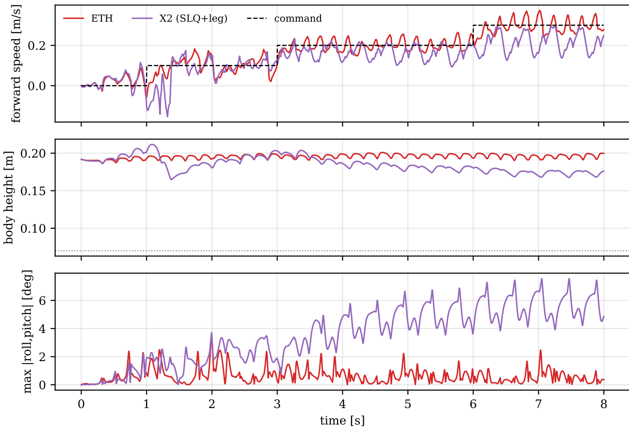
Dynamic tracking over the velocity staircase
