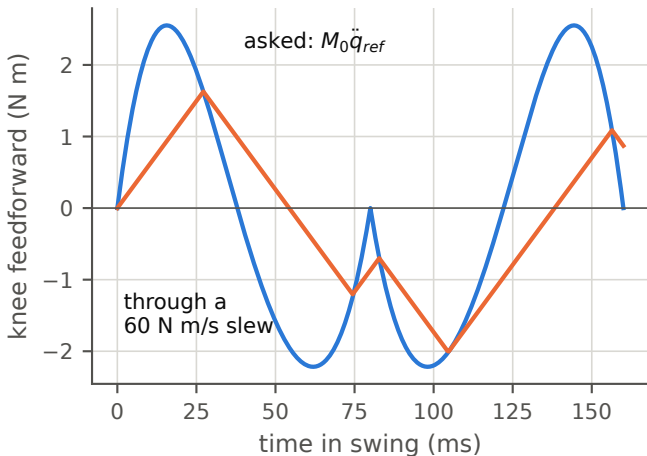
160 ms / 20 mm quintic arc
