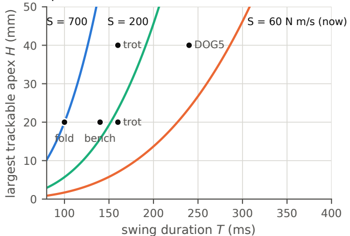
quintic arcs the slew lets the foot track
