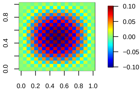
Vector 390
