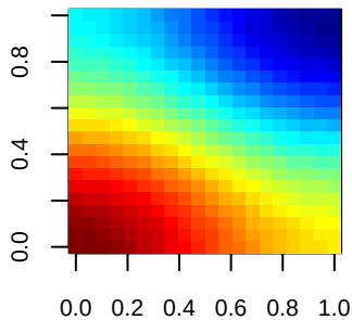
Vector 399
