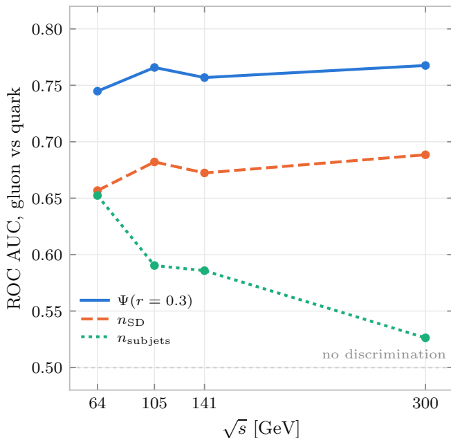
Figure 2. Area under the ROC curve as a function of centre-of-mass energy for the three discriminants, inclusive in \eta . The integrated jet shape and the iterated soft-drop multiplicity are stable across the range; the subjet multiplicity degrades towards the no-discrimination limit as \sqrt{s} grows.
