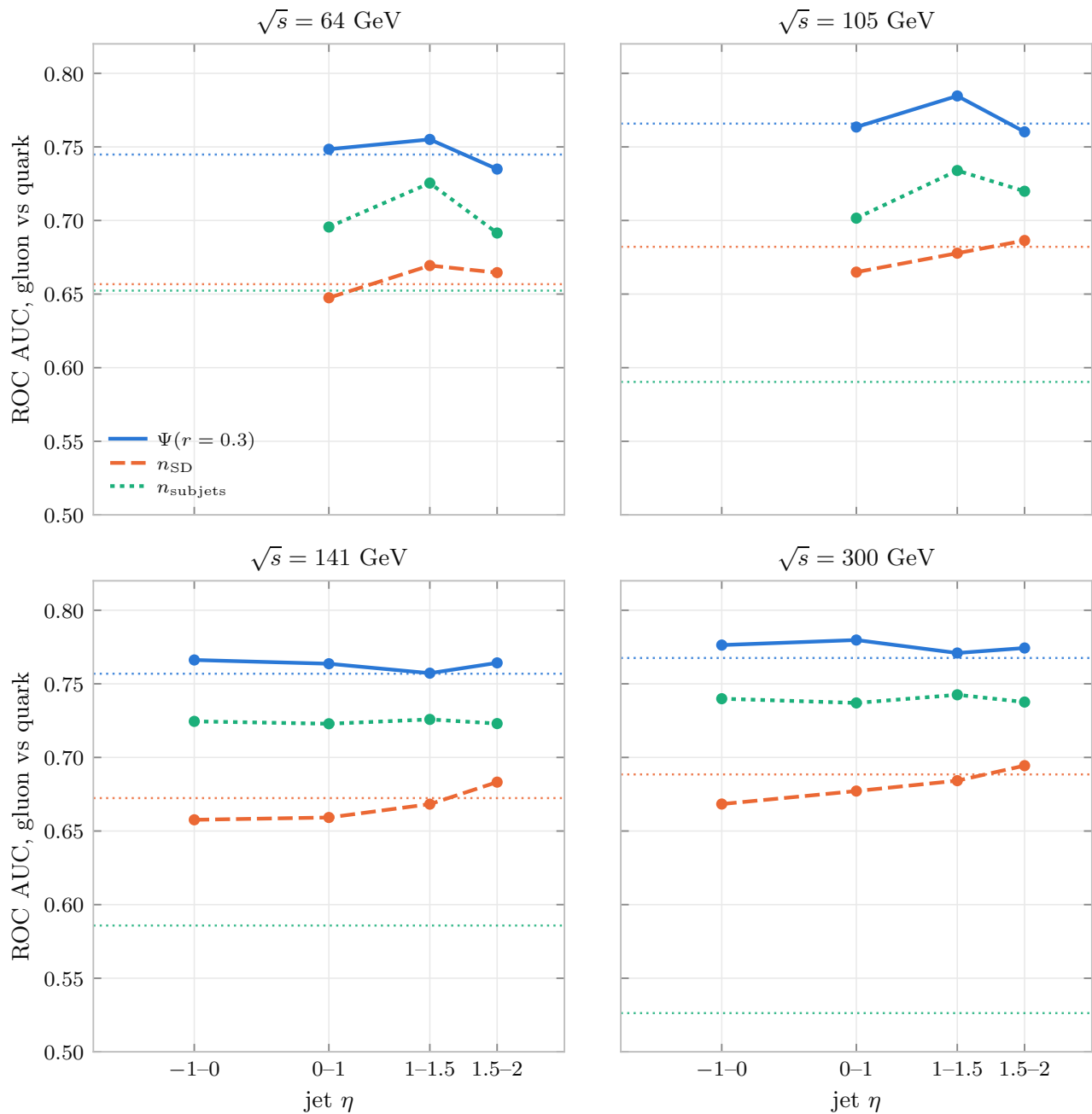
Figure 3. AUC in each pseudorapidity bin (markers) against the inclusive value for the same sample (dotted horizontal lines). \Psi(0.3) and n_{SD} are unaffected by pooling; n_{subjets} loses a large amount of discrimination to it. The \eta \in [-1, 0) bin is absent at 64 and 105 GeV, where the sample has too few jets there.
