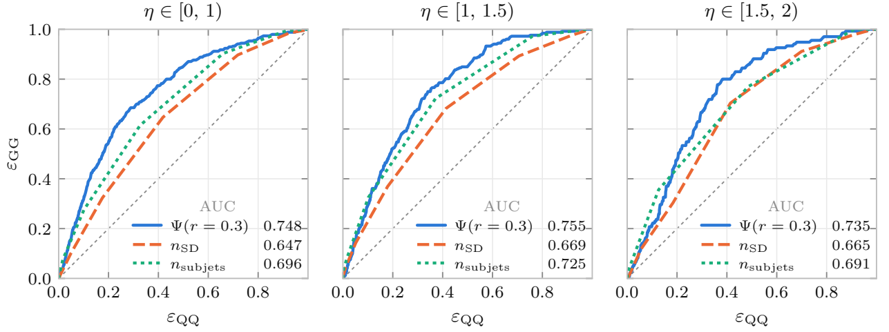
Figure 6. As Fig. 5, at \sqrt{s} = 64 GeV. The \eta \in [-1, 0) bin is omitted: it holds only ten GG jets.
