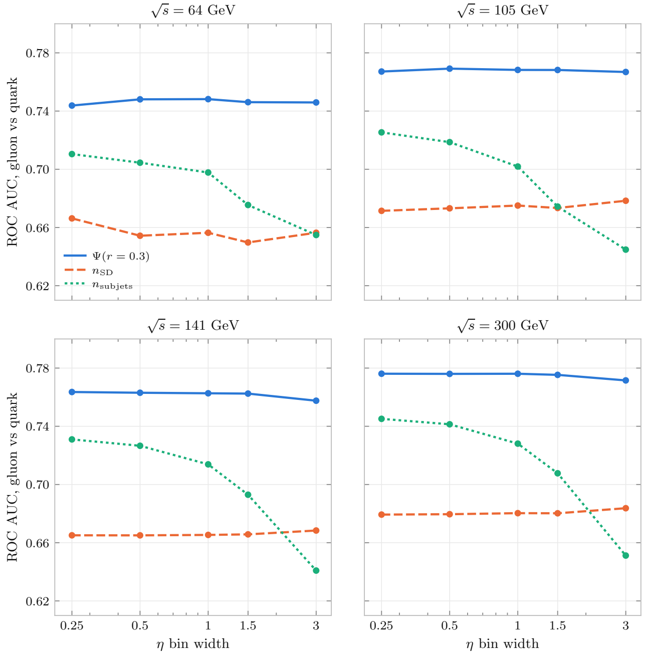
Figure 4. Jet-weighted mean AUC against \eta bin width, for uniform bins over -1 < \eta < 2 . A width of 3 is the pooled limit. \Psi(0.3) and n_{\text{SD}} are flat; n_{\text{subjects}} rises steadily as the bins narrow and overtakes n_{\text{SD}} near a width of 1.5.
