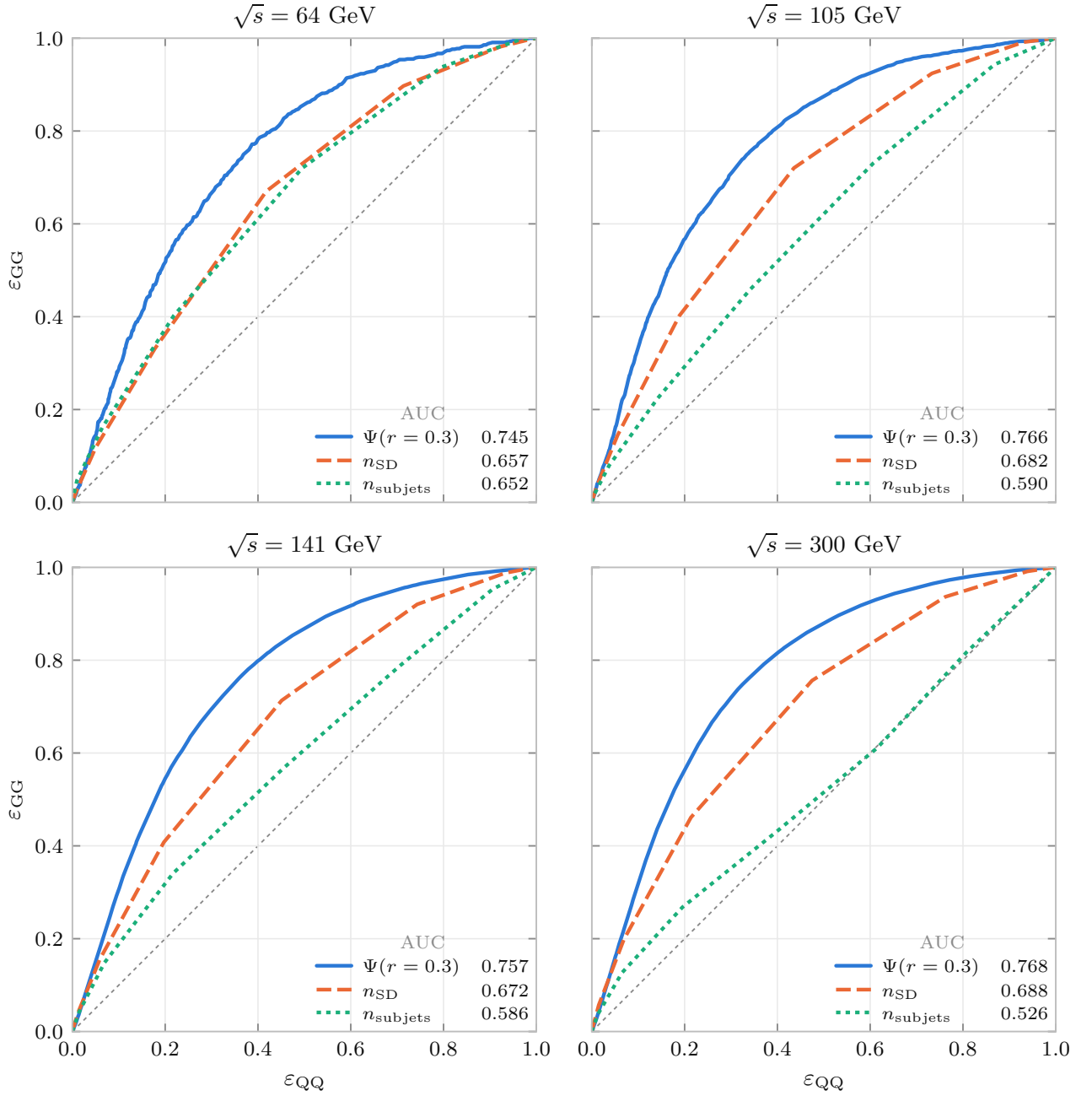
Figure 1. ROC curves for gluon-versus-quark discrimination at the four centre-of-mass energies. Signal is jets from GG events, background is jets from QQ events. All three observables are evaluated on identical jets (anti- k_T , R = 1.0 , exclusive two-jet, E_T > 10 GeV). The dotted diagonal is the no-discrimination limit. Legend entries give the area under each curve.
