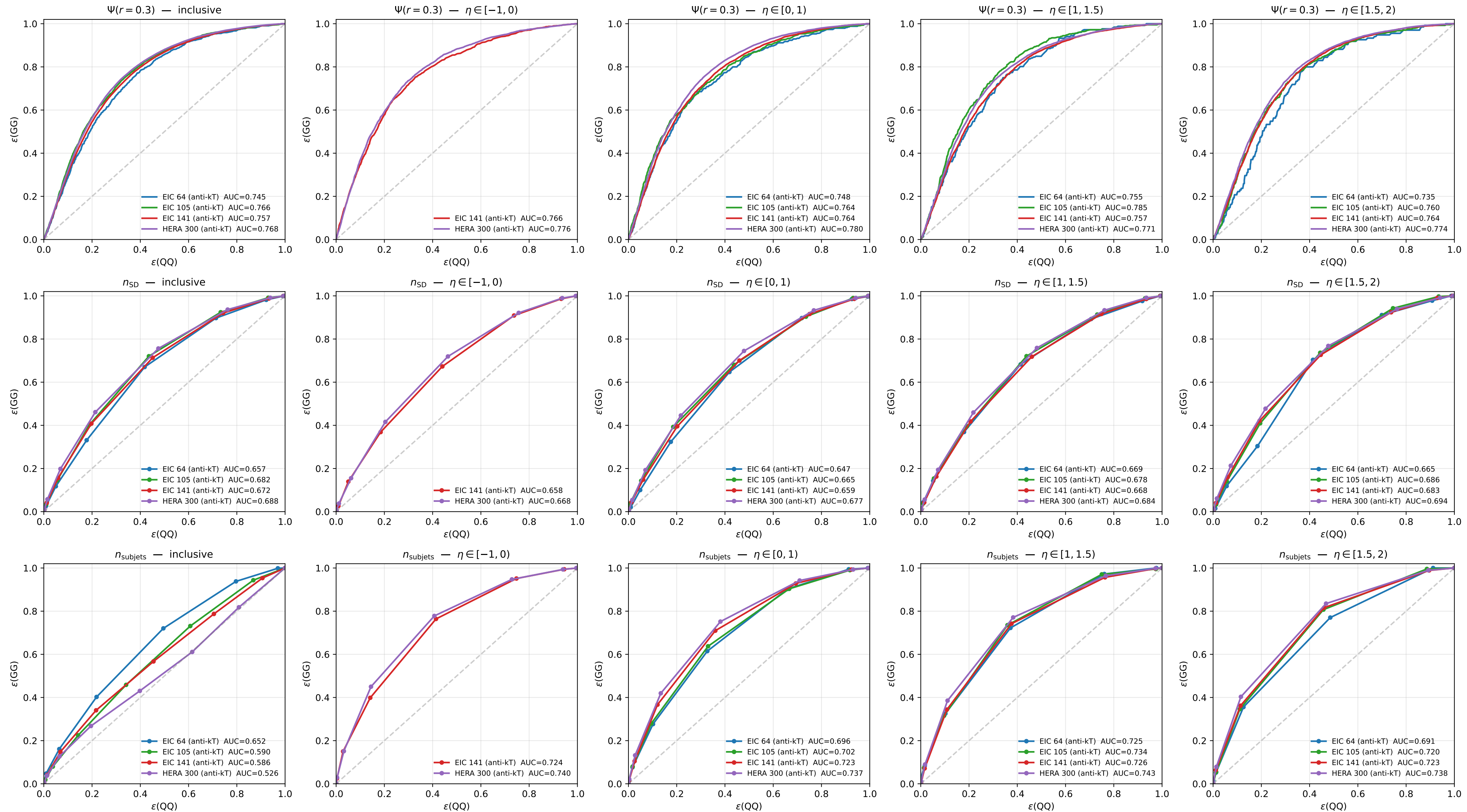
ROC curves across \eta bins and centre-of-mass energies (rows: \Psi(r=0.3) [top] / n_{SD} / n_{subjets} [bottom])
