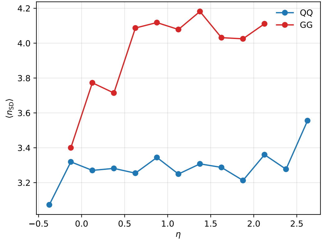
dijets_eic64_pTHat5_pT0Ref3.0_Q2max1_n1000k_R10_EtMin10_10j7
