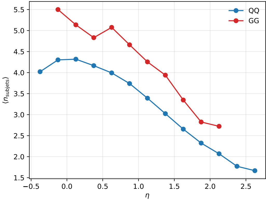
dijets_eic64_pTHat5_pT0Ref3.0_Q2max1_n1000k_R10_EtMin10_10j7
