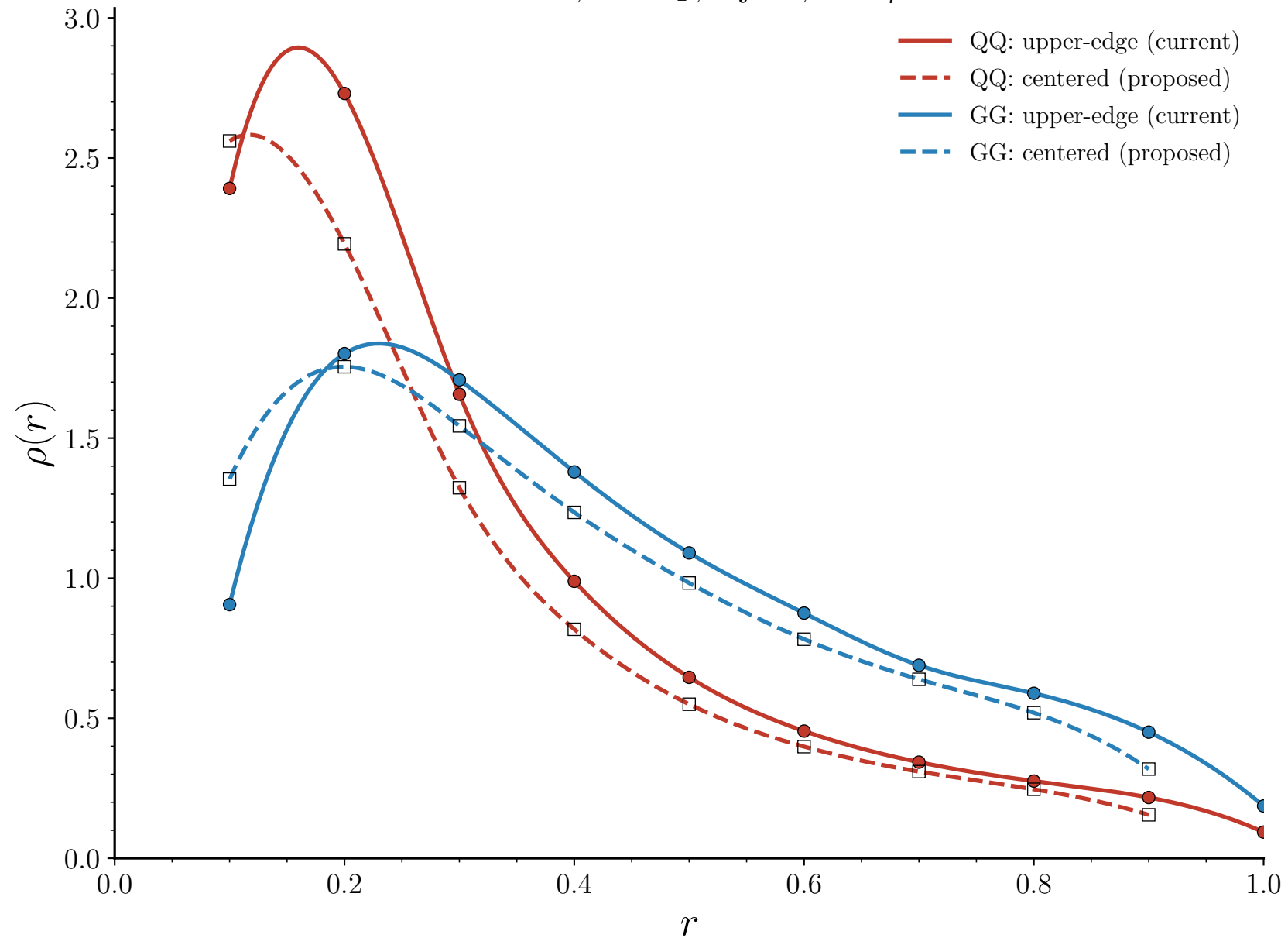
HERA 300, anti- k_T , dijets ; 0 < \eta < 1
