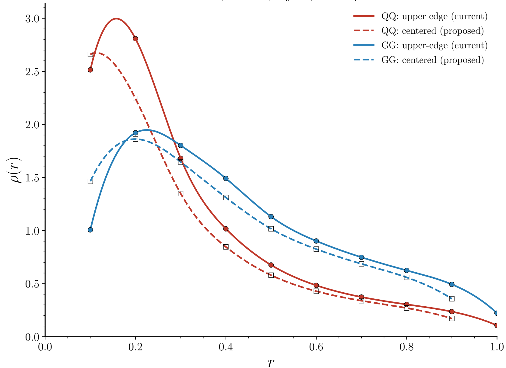
HERA 300, anti- k_T , dijets ; 1.5 < \eta < 2
