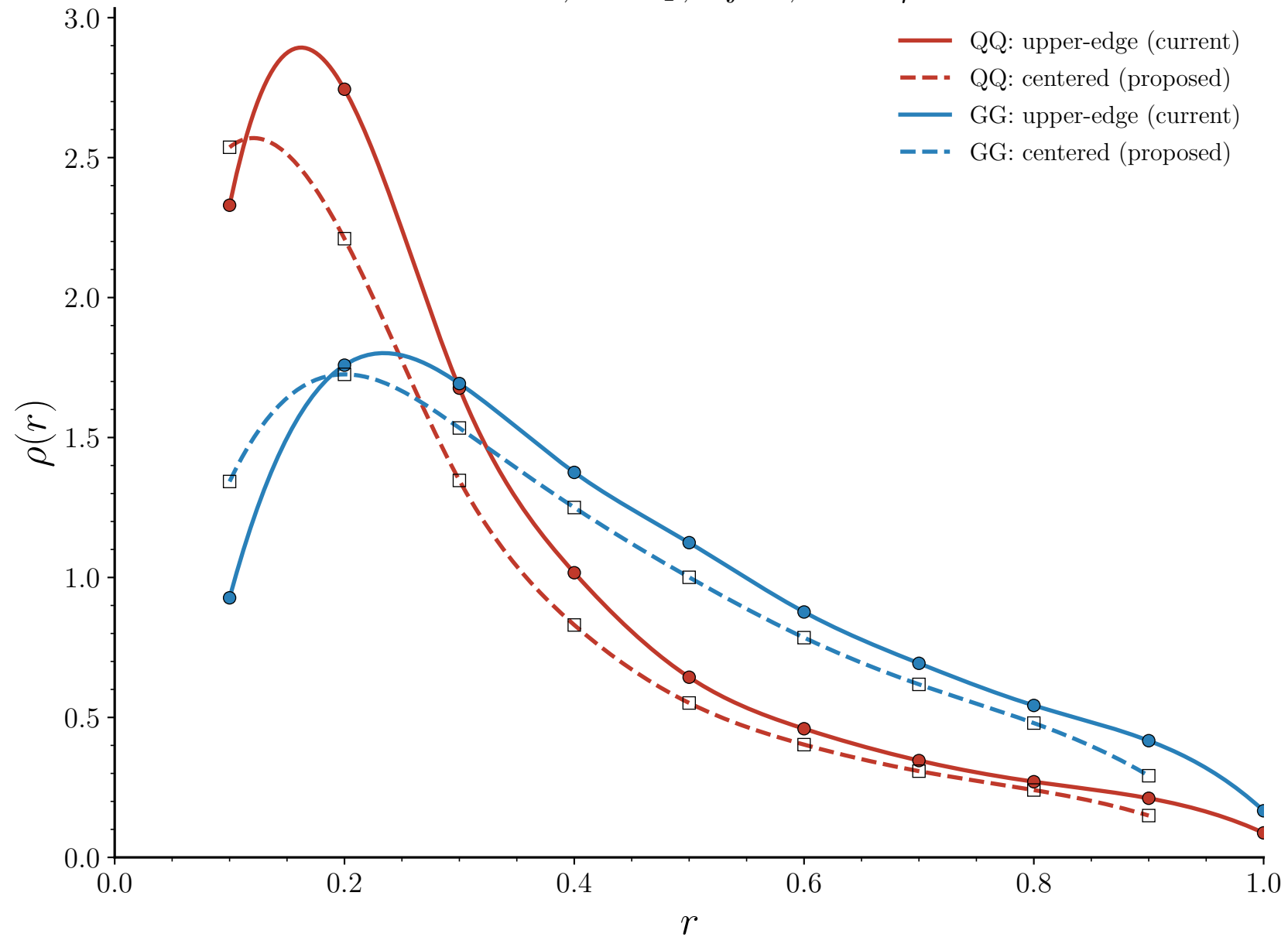
HERA 300, anti- k_T , dijets ; -1 < \eta < 0
