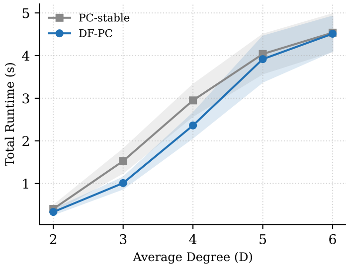
Graph=ER
