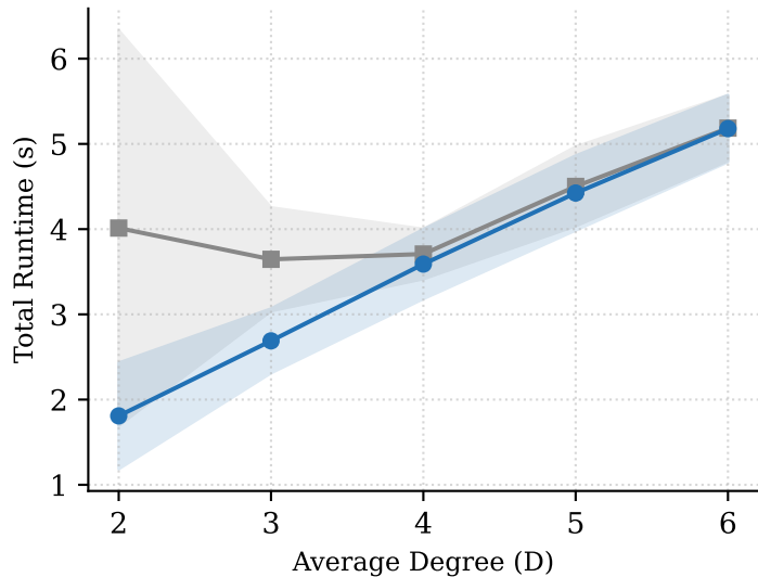
Graph=SF
