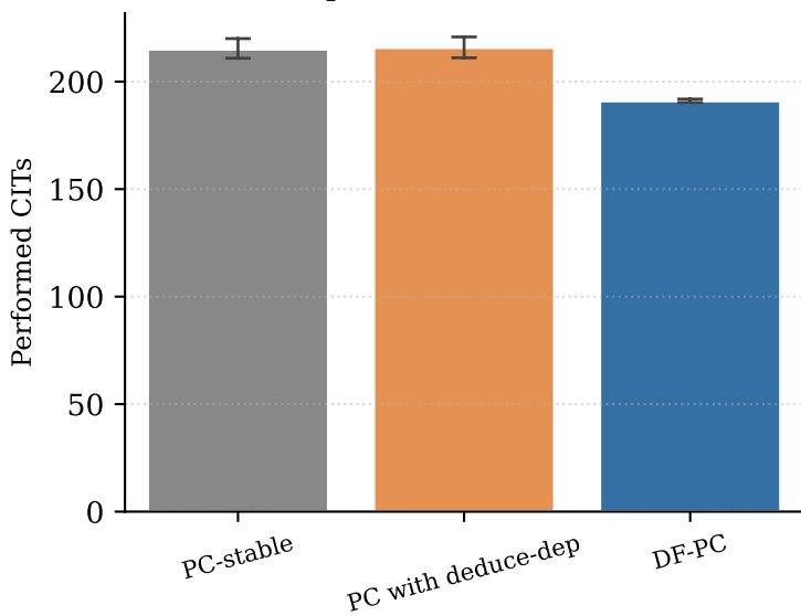
Graph=SF, Data=Discrete
