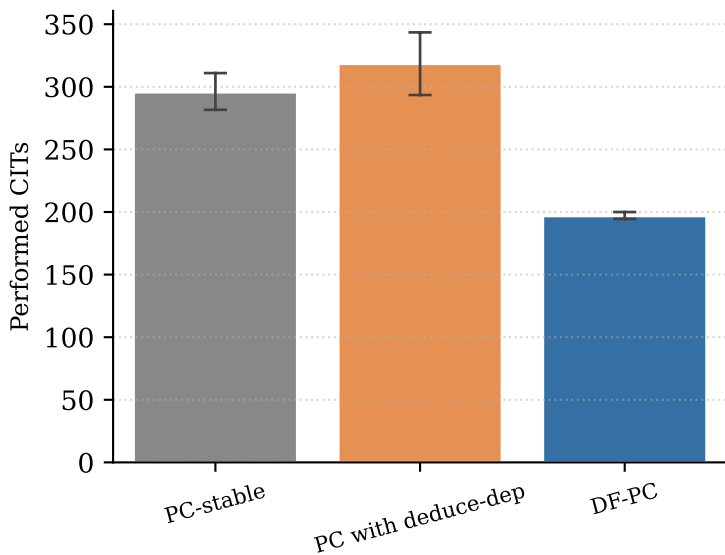
Graph=SF, Data=Discrete
