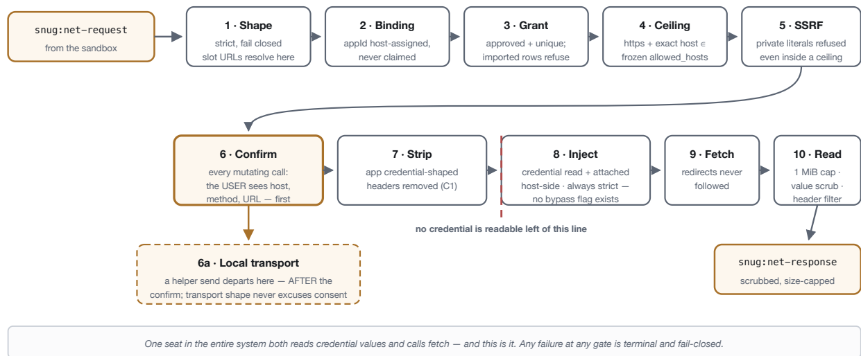
Figure 9. The executor's gate sequence. The confirmation gate precedes any credential read — a denied request resolves no secret and performs no fetch. A send to a local helper transport (§8) departs at gate 6a, after the confirmation and carrying the strip, injection, and scrub obligations with it; transport shape never excuses consent.
