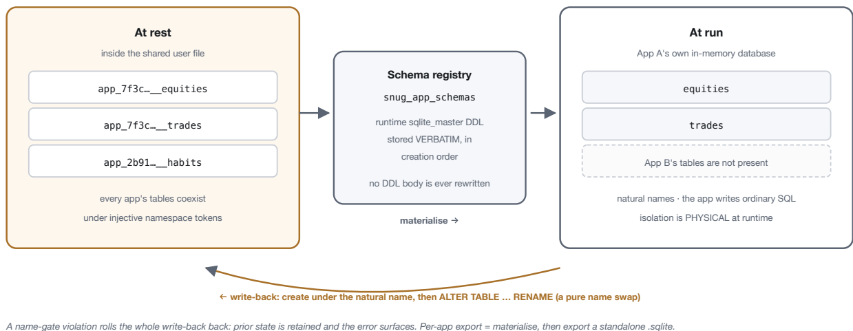
Figure 6. Materialisation. The registry stores each application's DDL verbatim; at load, those objects are replayed into a fresh in-memory database containing nothing else. The application executes ordinary SQL against natural table names, and isolation at runtime is physical rather than advisory.
