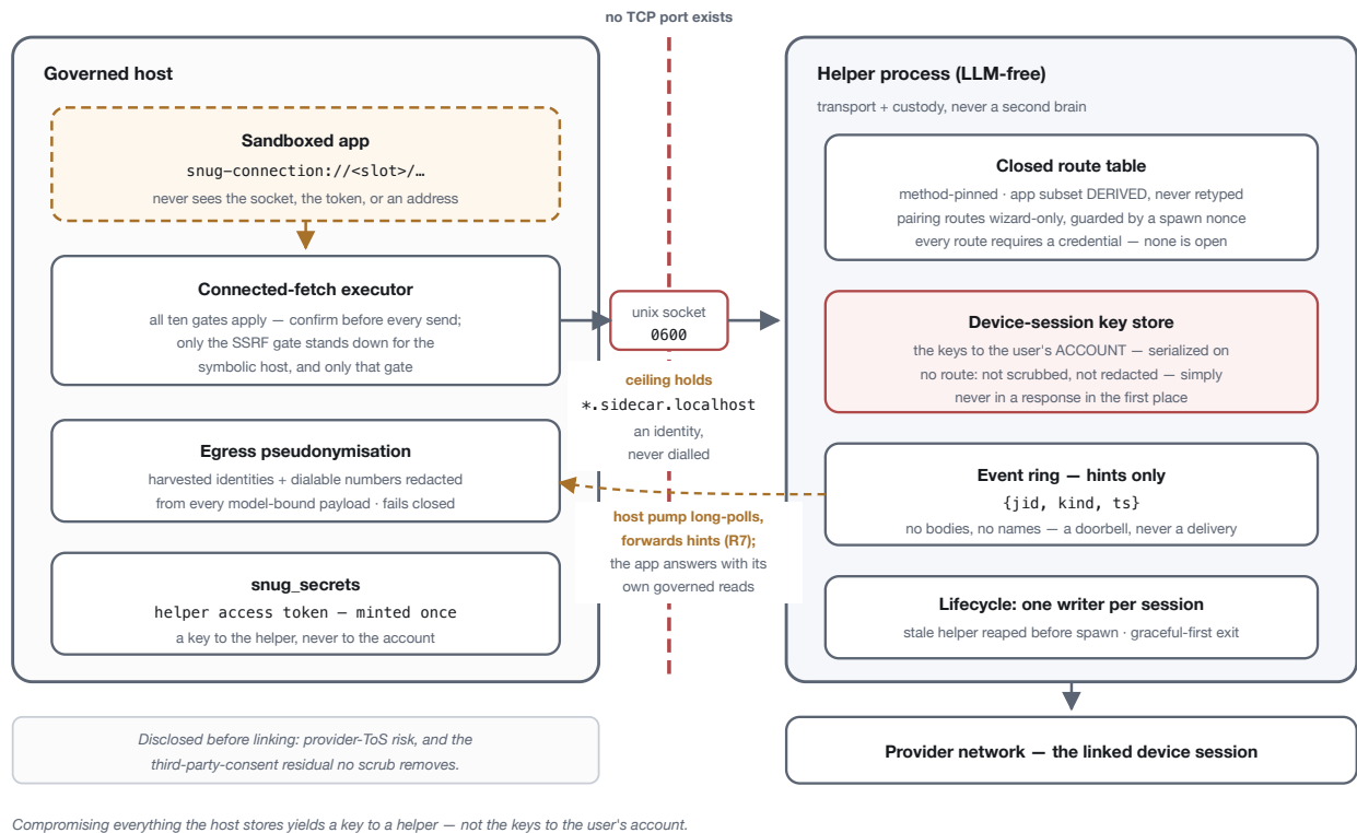
Figure 10. Linked-device connections. The application reaches the helper only through the governed executor; the ceiling holds a symbolic host that is an identity, never an address; the helper holds the device session's keys and serialises them on no route; pushes are hints (R7); and identities are pseudonymised before any model-bound payload leaves the host.
