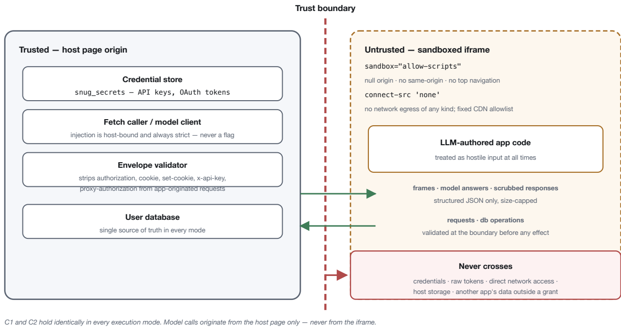
Figure 4. The trust boundary. Structured, size-capped JSON crosses in both directions and is validated before it can have any effect. Credentials, raw tokens, direct network access, and host storage never cross at all; other applications' data crosses only as rows under an access grant the user gave (§10).
