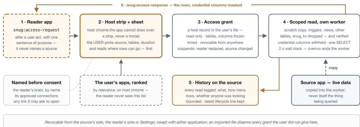
Figure 11. Access between apps. The reader asks; the user reviews on host chrome and picks the source and tables; the host writes the grant, copies the source into a scoped scratch database in its own worker, drops everything outside the grant, runs the one read under a wall clock, masks credential columns, logs the read on the source and hands the rows to the reader. The reader never sees the user's inventory; the source's live database is never queried.
