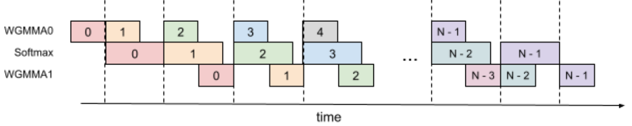
Figure 8: 3-Stage Pipelining
