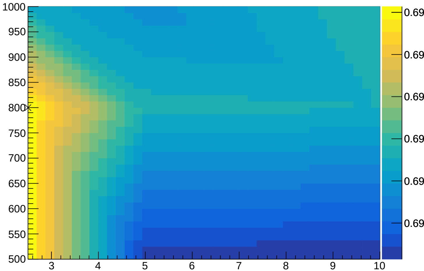
MinNodeSize:NTrees
