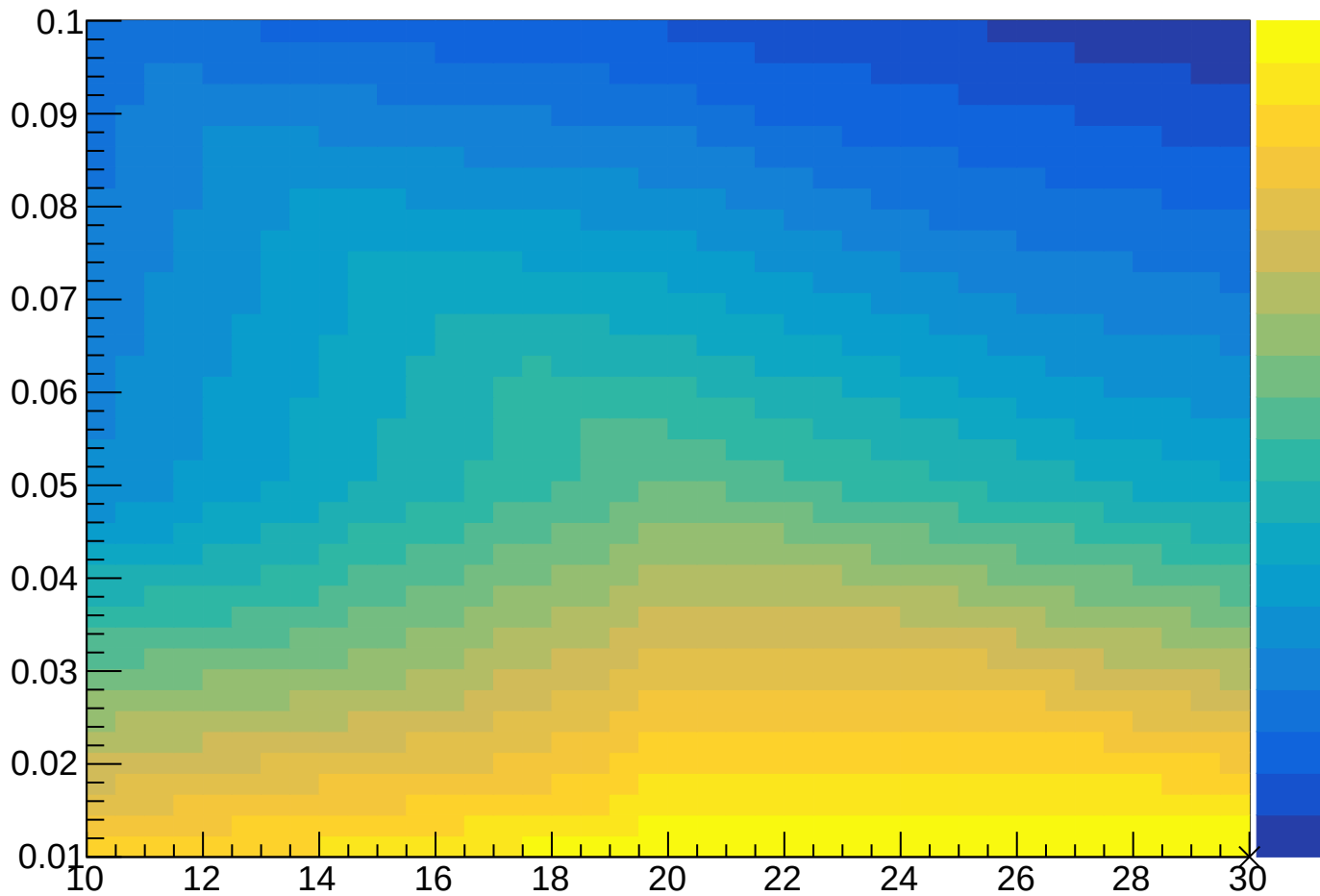
nCuts:Shrinkage
