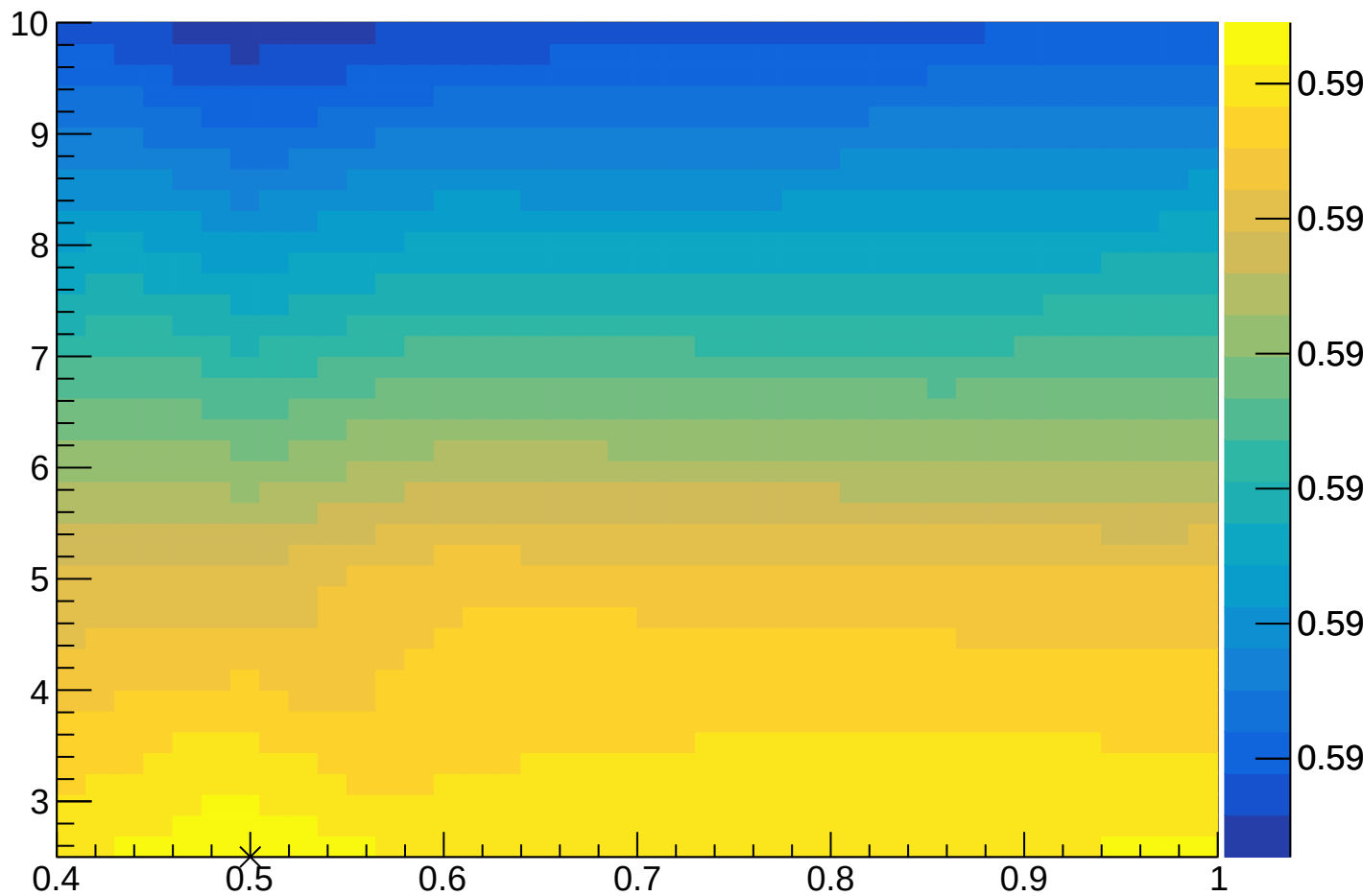
BaggedSampleFraction:MinNodeSize
