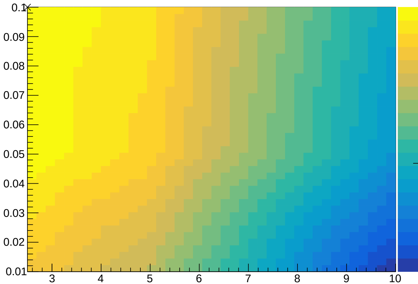
MinNodeSize:Shrinkage
