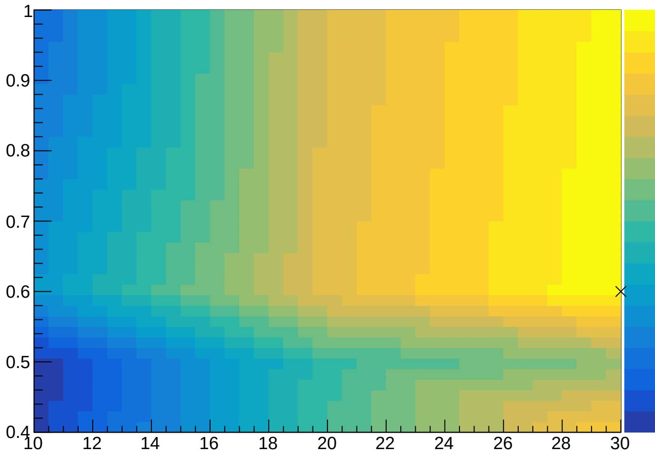
nCuts:BaggedSampleFraction
