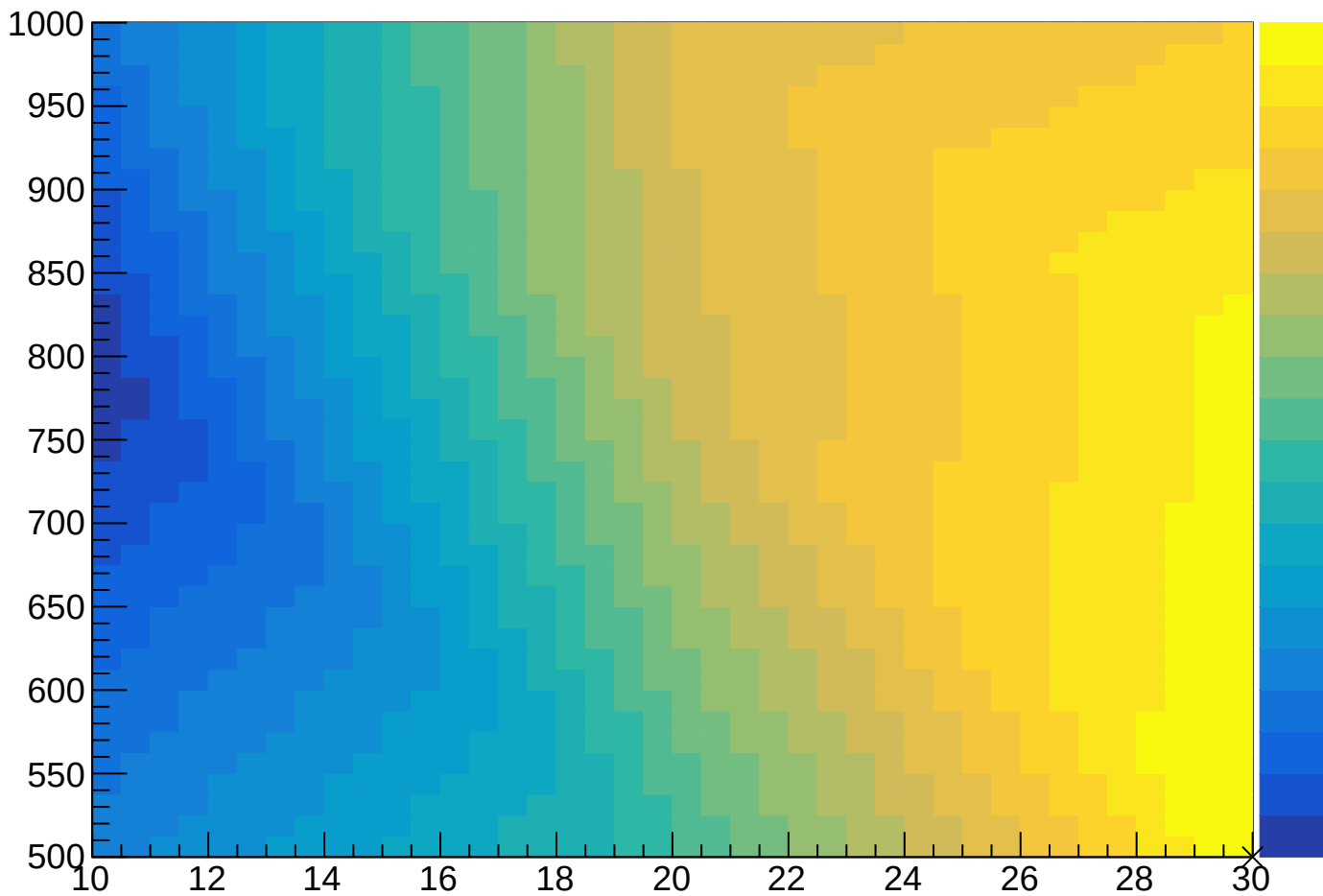
nCuts:NTrees
