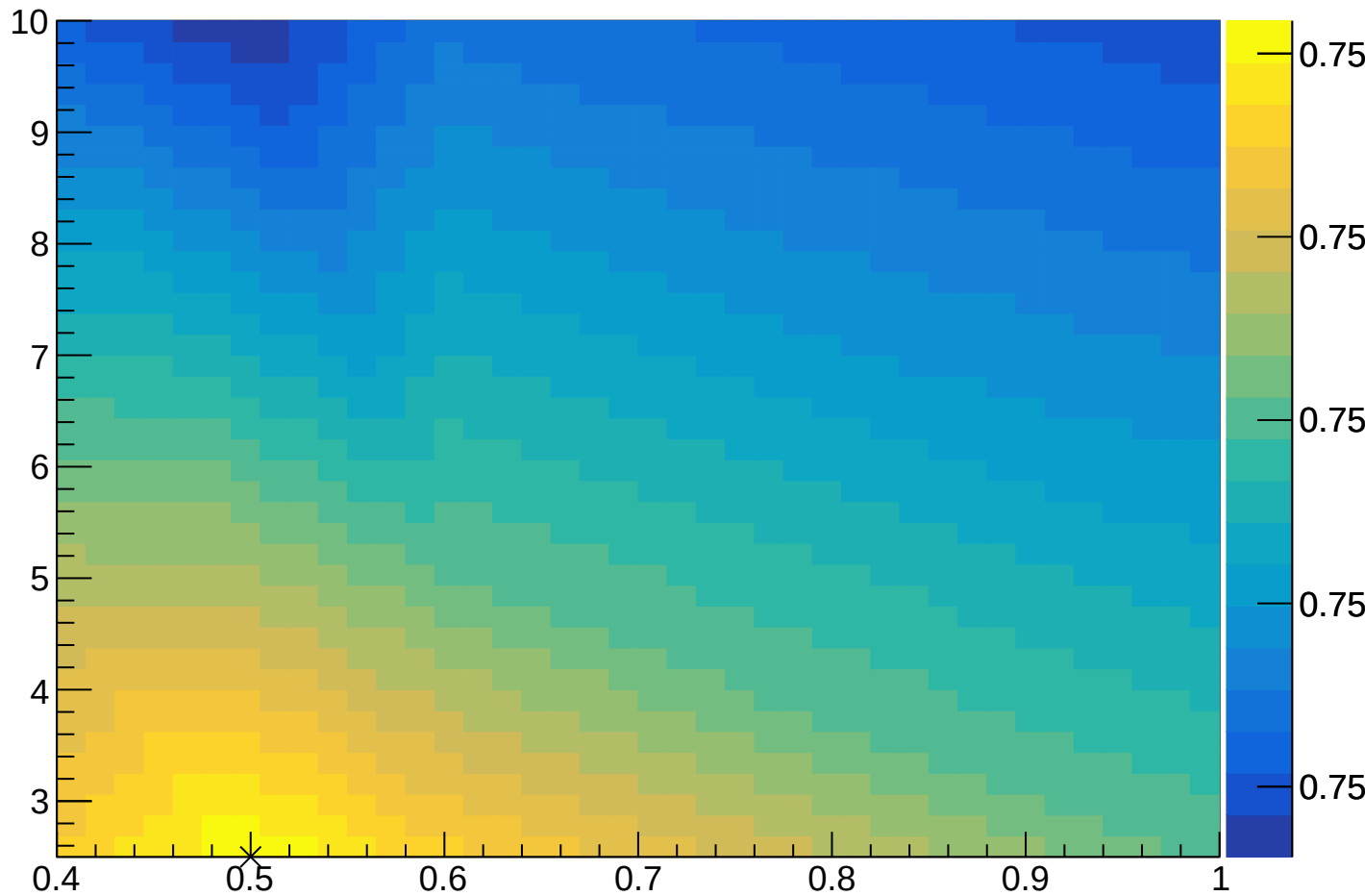
BaggedSampleFraction:MinNodeSize
