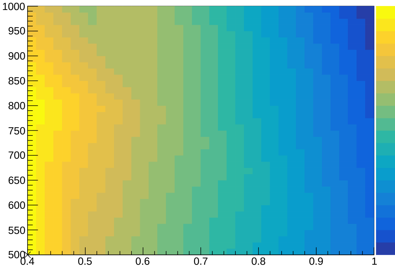
BaggedSampleFraction:NTrees
