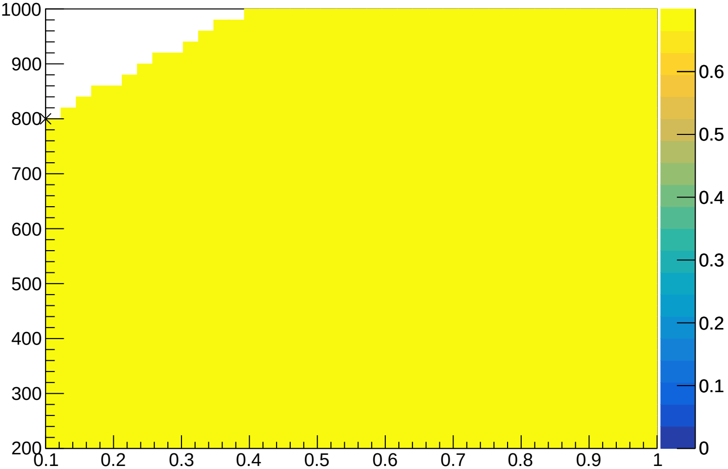
BaggedSampleFraction:NTrees
