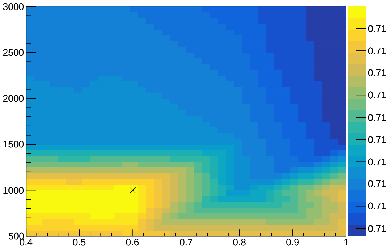
BaggedSampleFraction:NTrees
