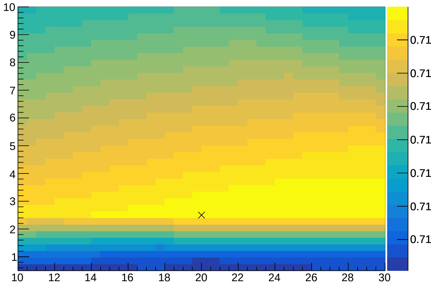
nCuts:MinNodeSize
