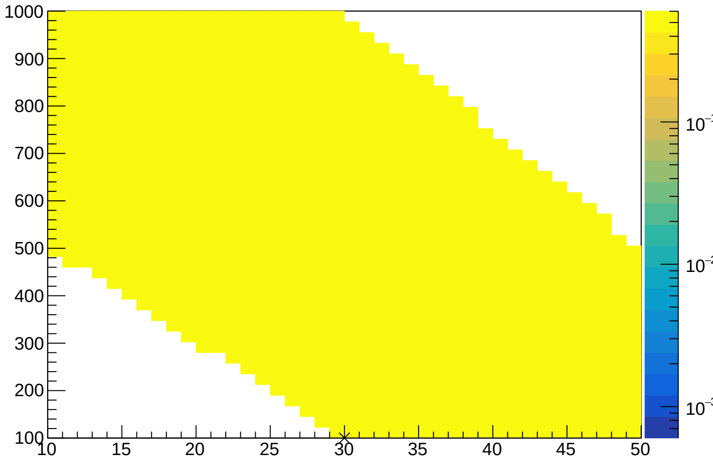
nCuts:Ntrees
