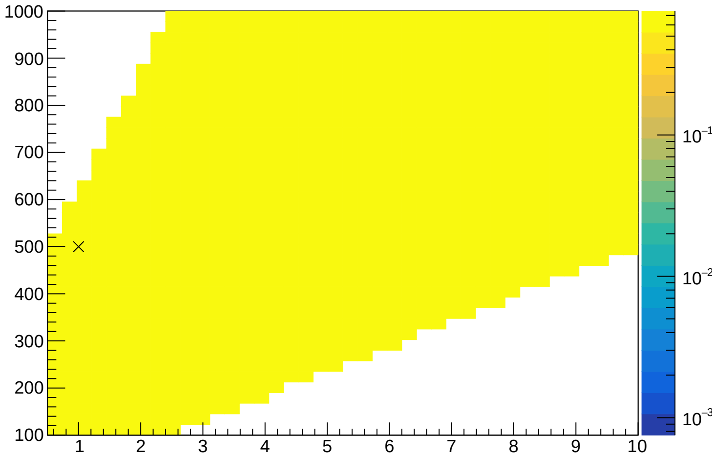
MinNodeSize:Ntrees
