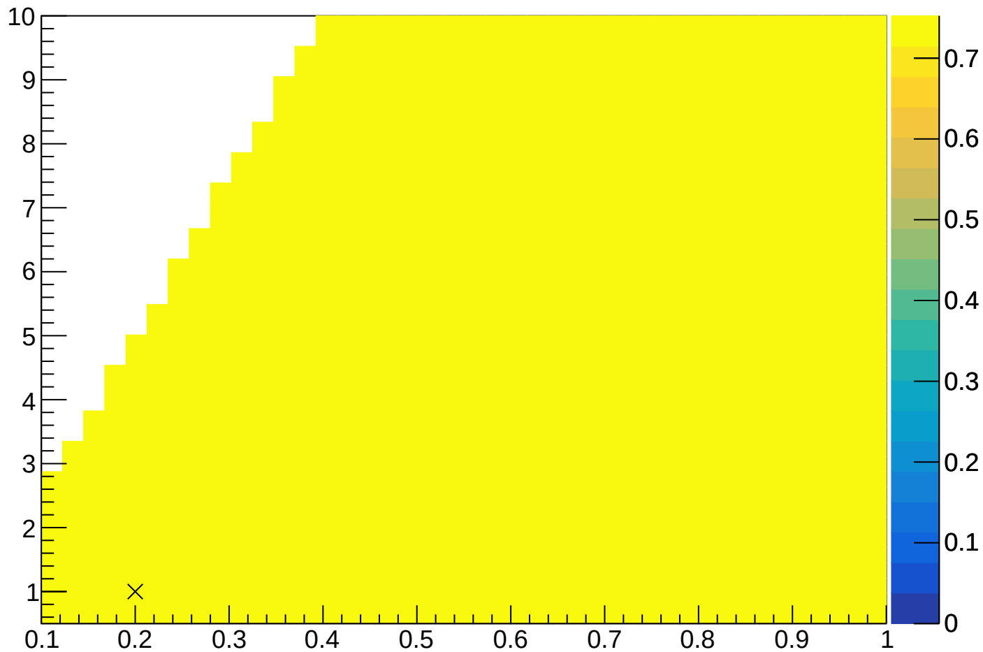
BaggedSampleFraction:MinNodeSize
