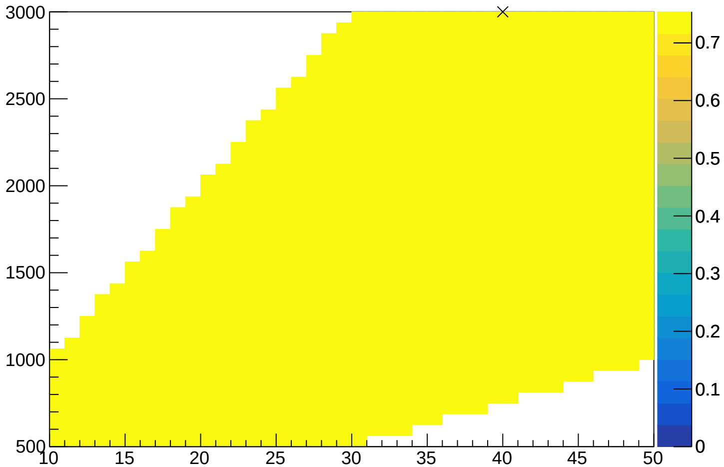
nCuts:NTrees
