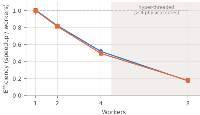
(b) Efficiency
