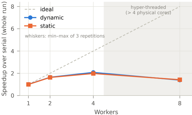
(a) Speedup
