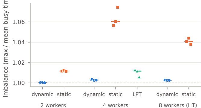
(b) Load imbalance
