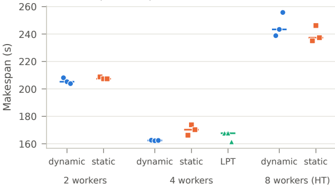
(a) Makespan, 3 repetitions (bar = median)
