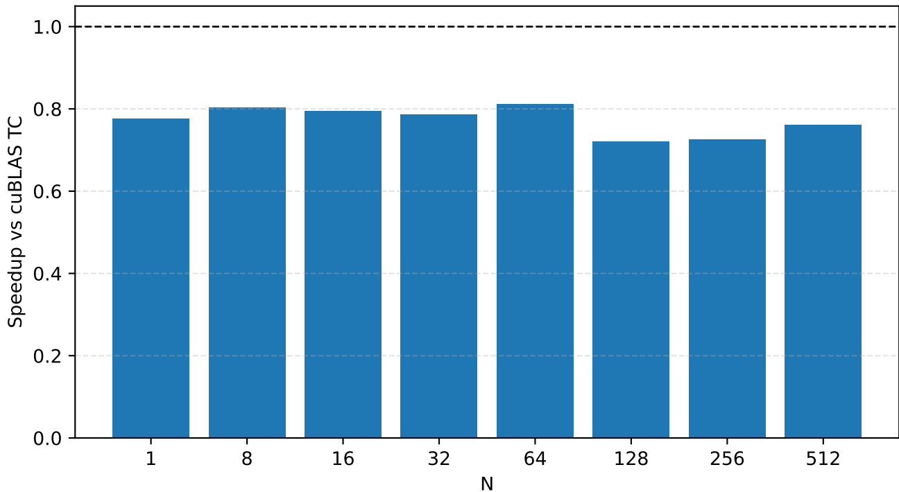
N sweep speedup, M=4096 K=4096 SplitK=1
